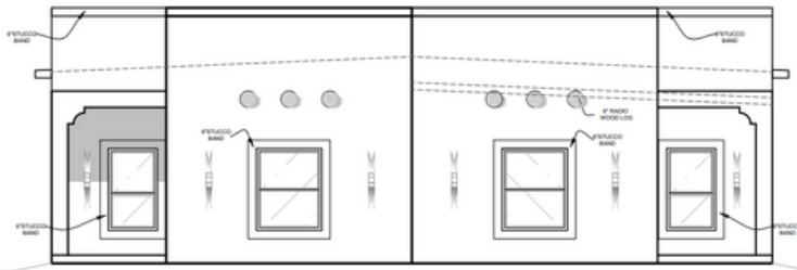
FRONT ELEVATION -SOUTHWEST B
